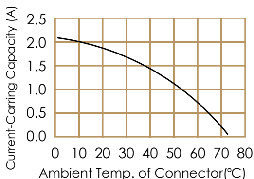
Figure 1 : Current Rating
