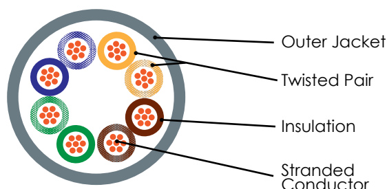
Figure 2 : Cable Structure
