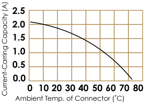
Figure 2: Current Rating
