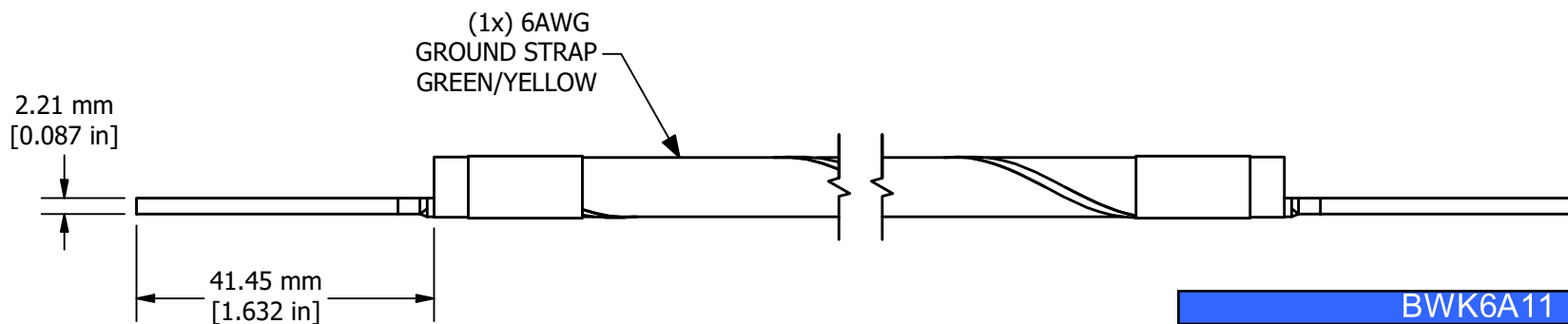
SIDE VIEW
