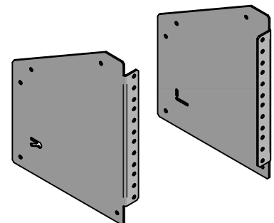
FIXED RAILS 1:6
