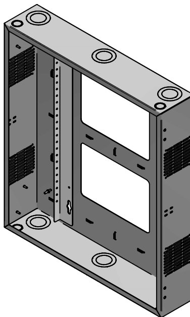
REAR SECTION 1:12
