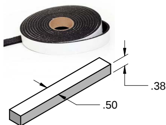
ITEM 6 - DOOR (PORTE) GSK 1/2" X 3/8" QTY: 2 @ 4.00" LG 1 @ 148" LG
