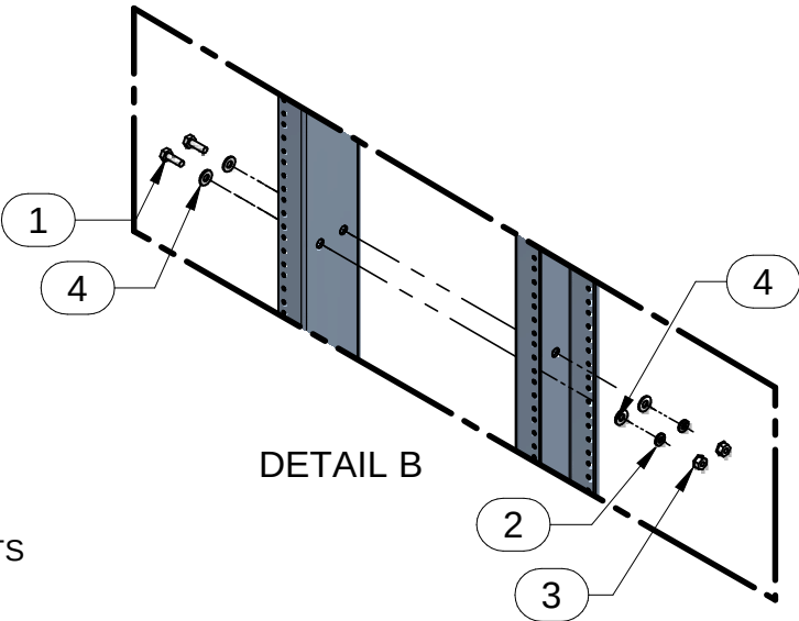
OPEN FRAME RACK GANGING DETAIL
