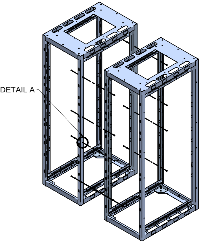
CABINET GANGING DETAIL
