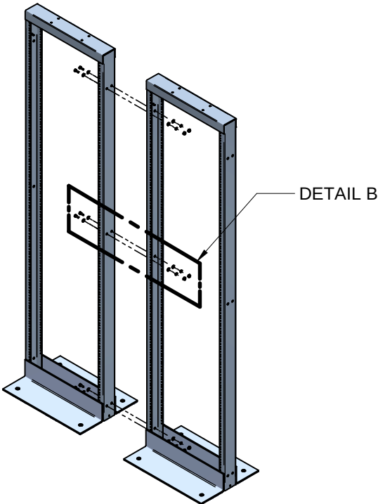
OPEN FRAME RACK GANGING DETAIL
