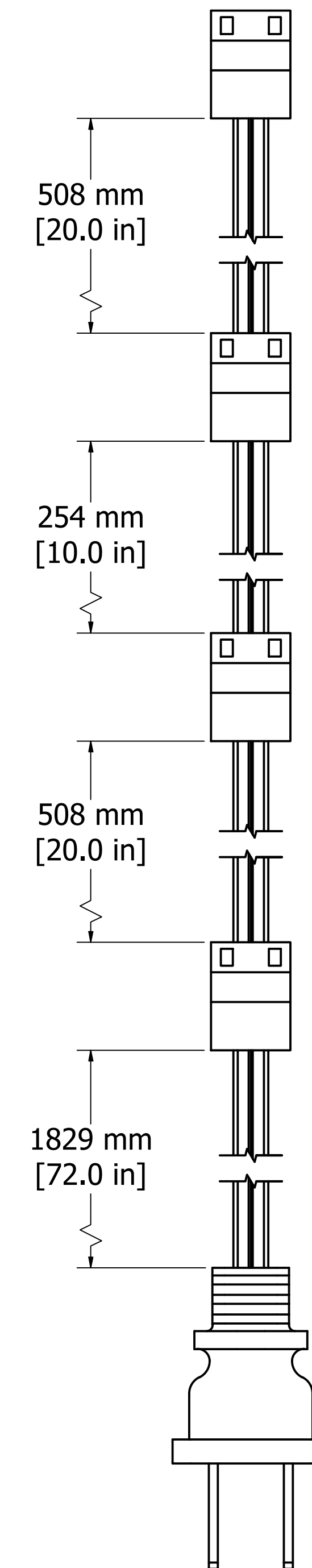
NEMA 1-15P DAISY CHAIN (4 FAN) CORD (1X)
