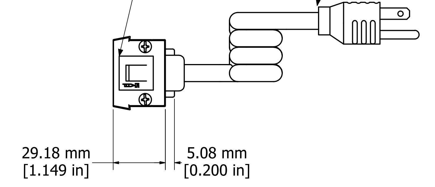
ASSEMBLY - VIEW FROM END
