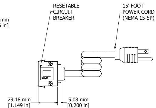
ASSEMBLY - VIEW FROM END
