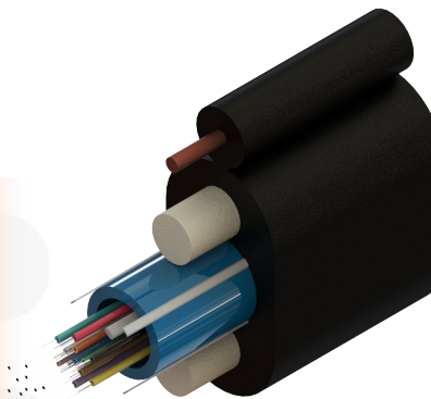
Toneable Flat Drop Cable (Simplex, Dual, Outdoor)
