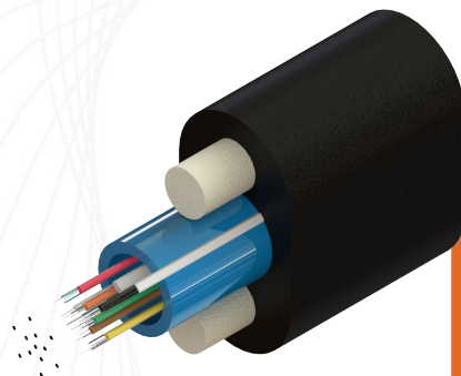
Flat Drop Cable (Dual, Outdoor)
