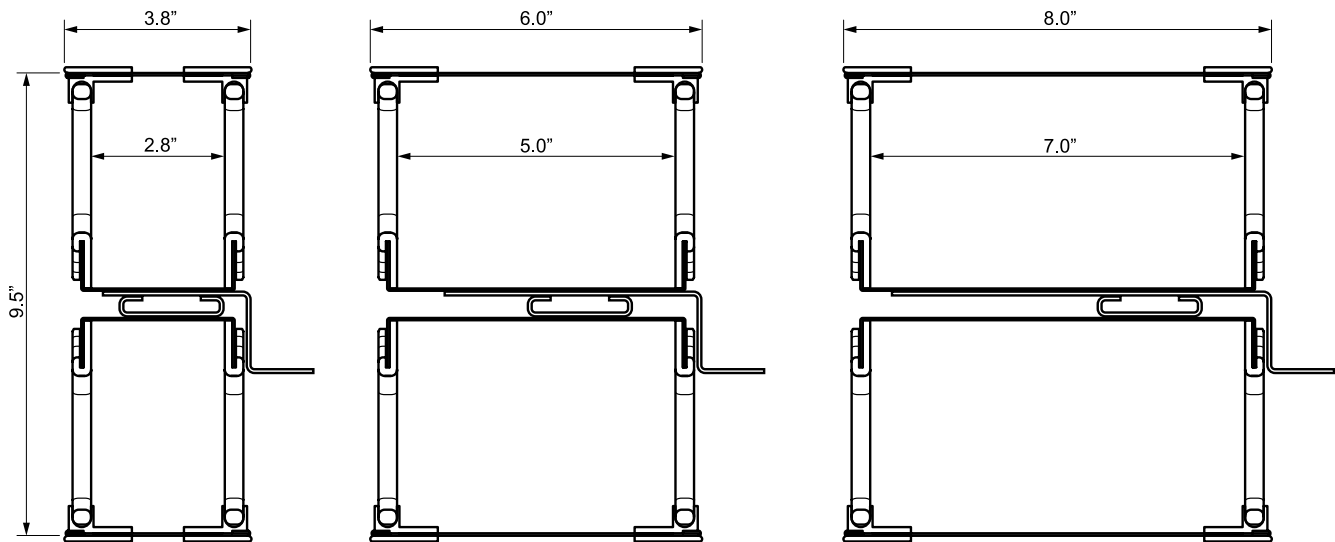
Technical Drawing- 2D Top View
